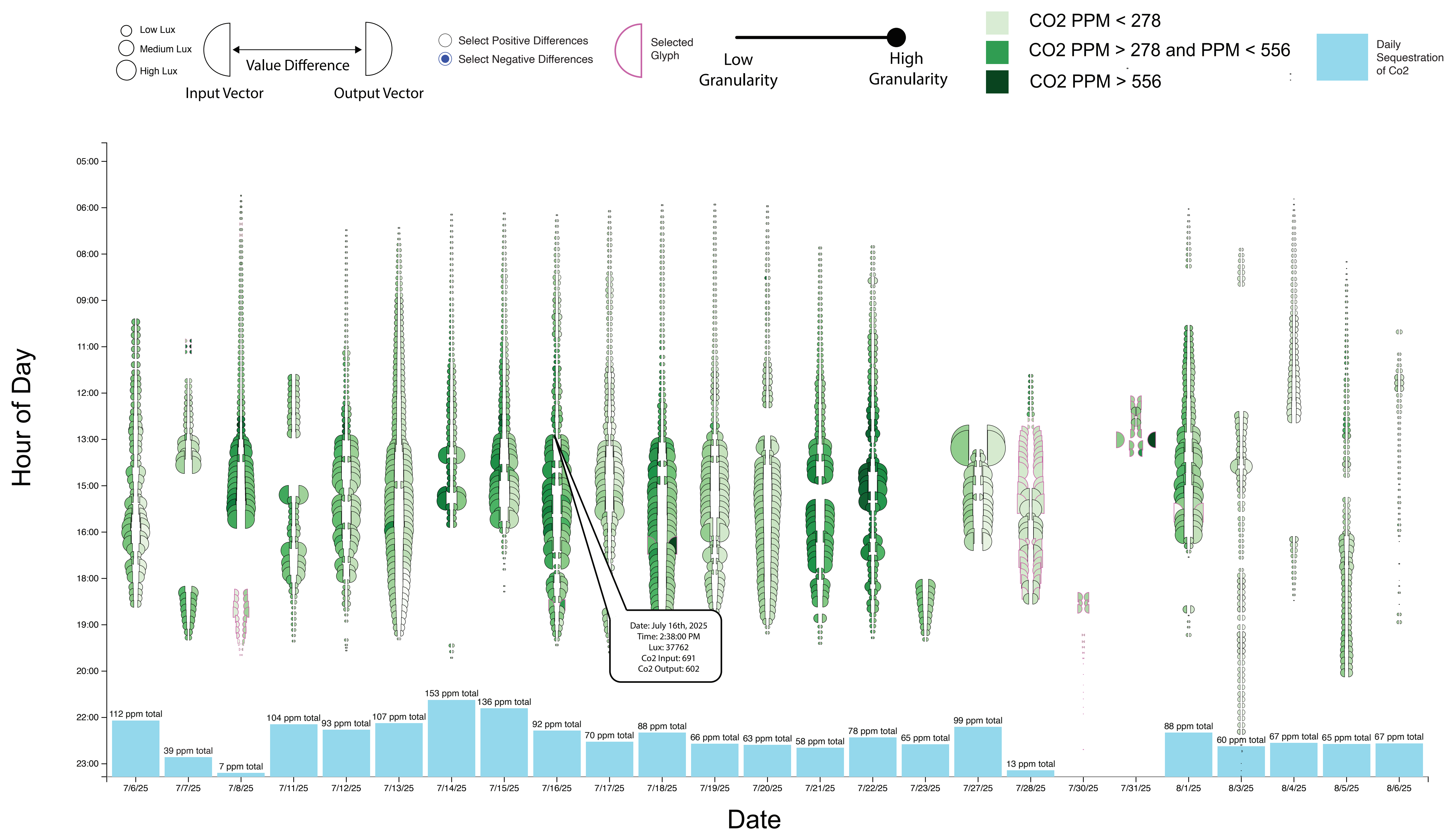
Figure 2: CO 2 input/output data and light data throughout July 2025 from bioreactors. The size of the semicircles encodes light values, while the color indicates concentration of CO 2 . The distance between the two semicircles represents the difference in CO 2 input and output, with negative differences highlighted in magenta. The height of the bar at the bottom encodes daily aggregated CO 2 sequestration. The figure reveals the bioreactor sequesters the most CO 2 in the afternoons when sunlight is most intense.
